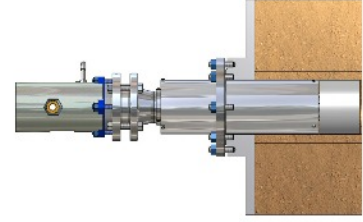
6F - 6", 150# CLASS FLANGE MOUNT CONFIGURATION
